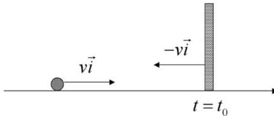
Fig. 7.1. Elastic collision at time t = t_0
