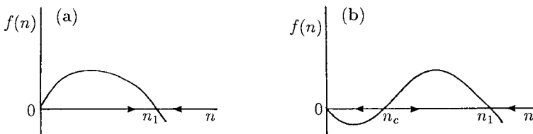
Figure 11.4. (a) Typical firing rate function f(n) with a single nonzero steady state: n \rightarrow n_1 in the absence of spatial effects. (b) A typical multi-steady state firing function. If n < n_c , a critical firing rate, then n \rightarrow 0 , that is, extinction. If n > n_c then n \rightarrow n_1 .
