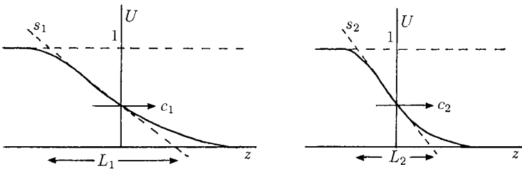
Figure 13.3. Steepness s (= |U'(0)|) and a practical measure of the width L (= 1/s) for wavefront solutions of the Fisher–Kolmogoroff equation (13.6) for two wavespeeds, c_2 and c_1 > c_2 \geq 2 . The flatter the wave the faster it moves.
