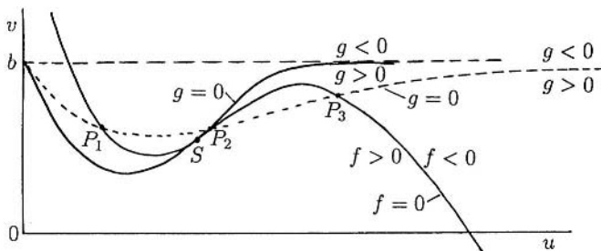
Figure 6.8. Schematic null clines for the substrate–inhibition kinetics (6.117). There may be one, S , or three, P_1, P_2, P_3 (dashed g = 0 curve) steady states where f = 0 and g = 0 intersect. Note the signs of f and g on either side of their null clines.
